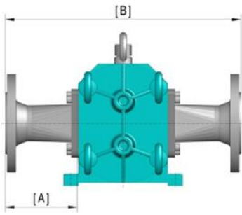
Design 1 | Short, straight pipe connectors with connection flange and gasket, in mm (approx.)
