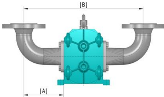
Design 2 | 90° elbow up in mm (approx.)
