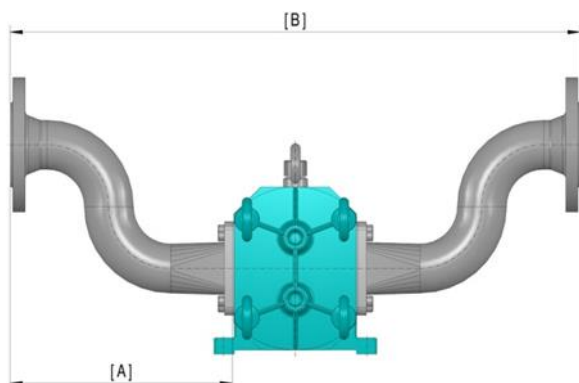
Design 6 | Gooseneck version in mm (approx.)
