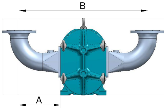
Bauform 2 90° Bogen oben in mm / inches Design 2 90° elbow up in mm / inches
