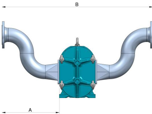
Bauform 6 Schwanenhals-Ausführung in mm Design 6 Gooseneck version in mm / inches
